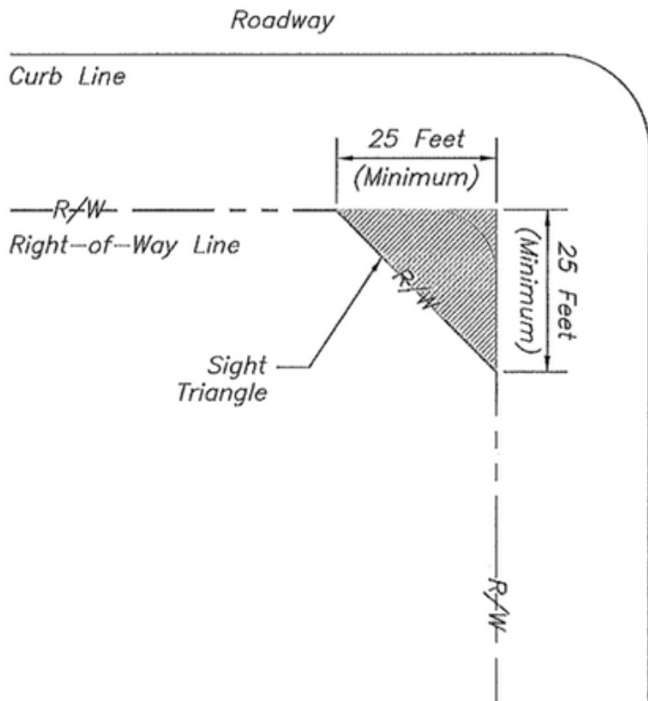
Exhibit 240.33: Sight Triangle
